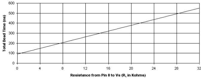
A121 Typical Total Dead Time As A Function Of Resistance From Pin 8 to +5 Volts DC
