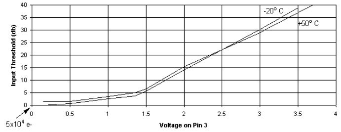
A121 Input Threshold Vs. Control Voltage on Pin 3 (at +50° C and -20° C)
