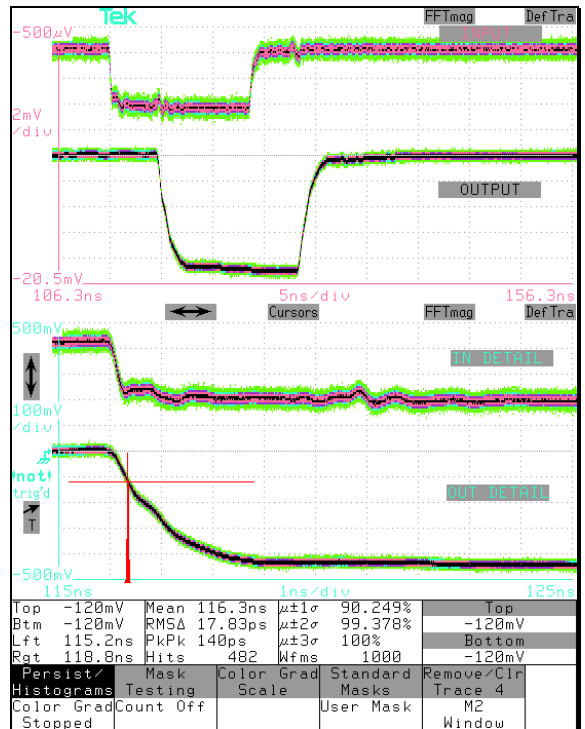
AM8303 BWL (x100), Input 2mV/div, Output 100mV/div
