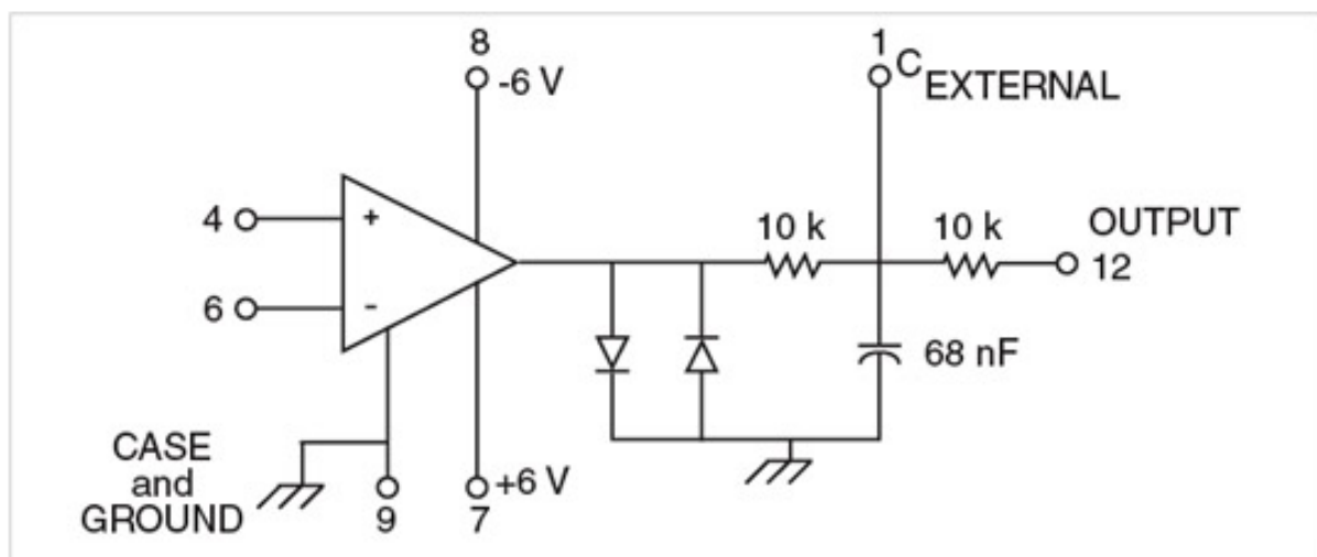
BLR1 PIN CONFIGURATION
